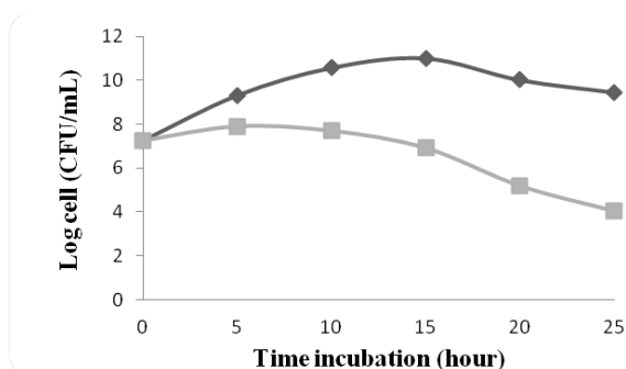
Figure 4. Growth pattern of UPEC; control (■), treatment by FU3 infection (■)
