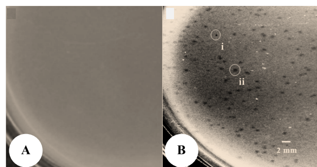
Figure 1. UPEC culture in double layer agar which was incubated at 37°C for 24 h: A. Without phage infection; B. With phage infection that resulted in various plaque size: FU1 (i), FU3 (ii)
