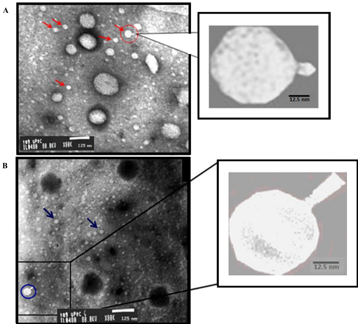
Figure 2. TEM image with negative staining by 2% uranyl acetate in magnification of 80000×: A. FU1 phage, B. FU3 phage
