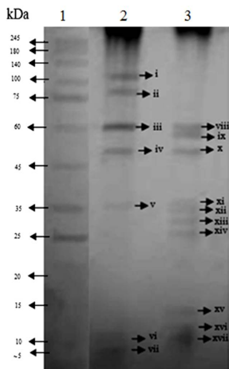
Figure 3. Protein molecule weight ranges in 10% concentration of SDS-PAGE: 1. Marker (SMOBIO PM 2700); 2. FU3: 120 kDa (i), 99 kDa (ii), 74 kDa (iii), 54 kDa (iv), 36 kDa (v), 11 kDa (vi), 8 kDa (vii); 3. FU1: 76 kDa (viii), 60 kDa (ix), 52 kDa (x), 37 kDa (xi), 32 kDa (xii), 30 kDa (xiii), 28 kDa (xiv), 13 kDa (xv), 11 kDa (xvi), 10 kDa (xvii)
