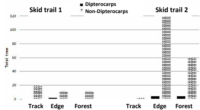
Figure 5. Dominant tree family in skid trail 1 and 2.
